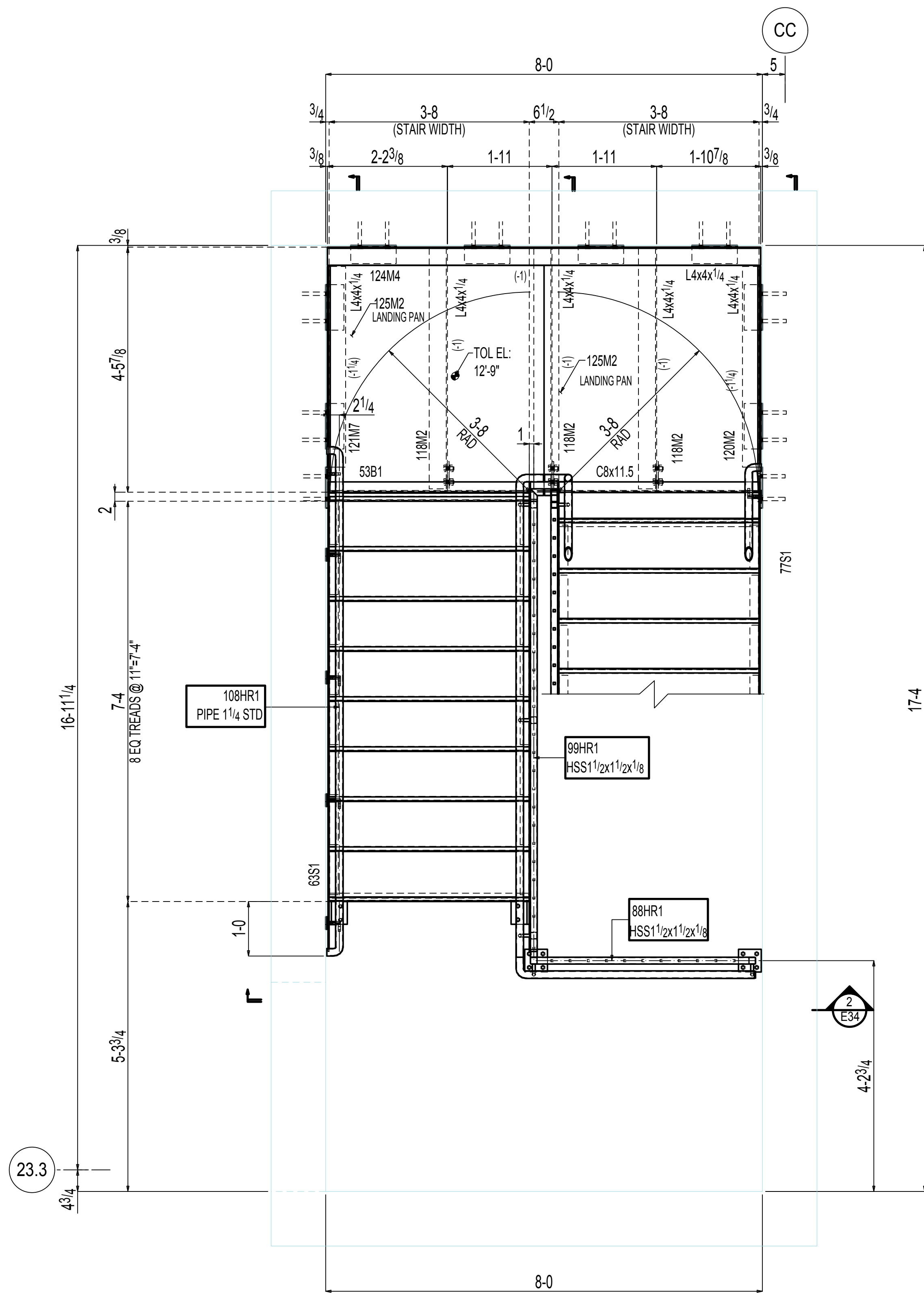
STAIR -1 PLAN (REF DWG:A601) NOTES: 1. TOP OF STEEL ELEVATION = (12-6) U.N.O. 2. (+/- X-X) = ABOVE/BELOW TOP OF STEEL ELEVATION.
