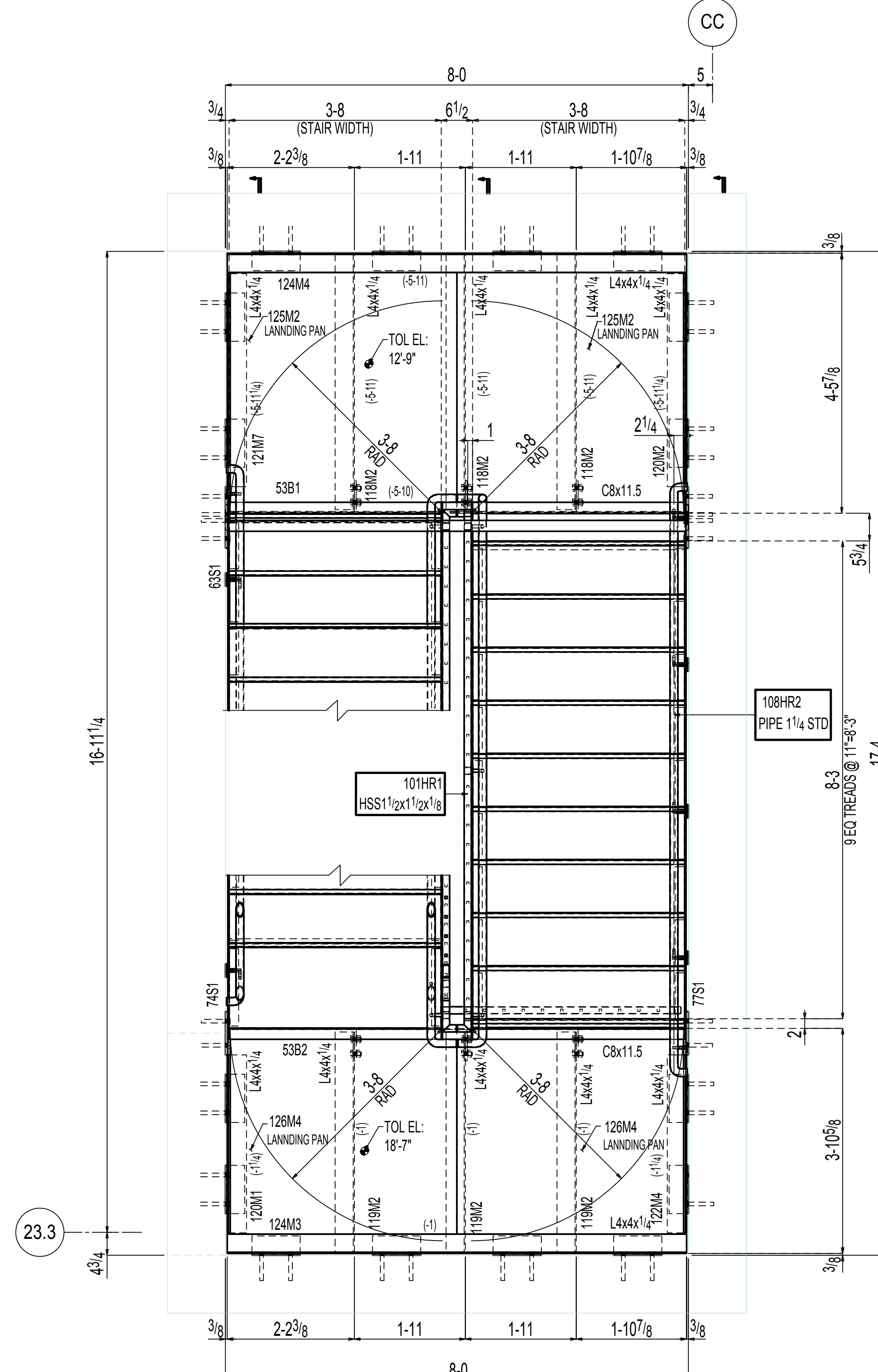
STAIR -1 PLAN (REF DWG:A601) NOTES: 1. TOP OF STEEL ELEVATION = (18-4) U.N.O. 2. (+/- X-X) = ABOVE/BELOW TOP OF STEEL ELEVATION.
